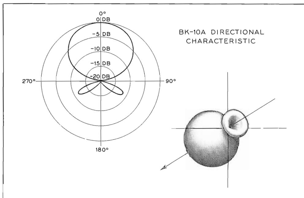
FIG. 1. At left, the conventional drawing shows the bigradient characteristics of the BK-10A. On the right, this bigradient characteristic is shown in a three dimensional configuration.
