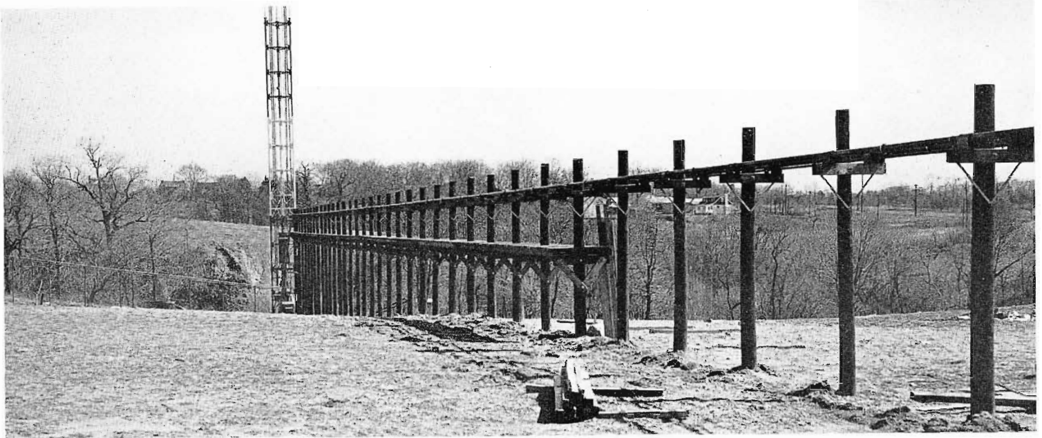
FIG. 6. WFIL constructed these support posts for the new 3 1/8-inch Universal Transmission Line. The line runs approximately 600 feet from the WFIL building.
