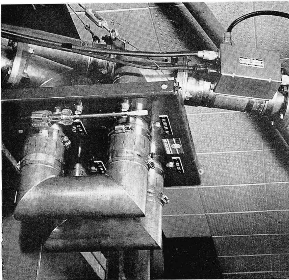
FIG. 3. Manual coaxial switching panel permitted rapid manual switching between 1 and 12 kilowatt outputs during conversion, and ultimately between 1 and 25 kilowatt outputs after conversion was completed.
