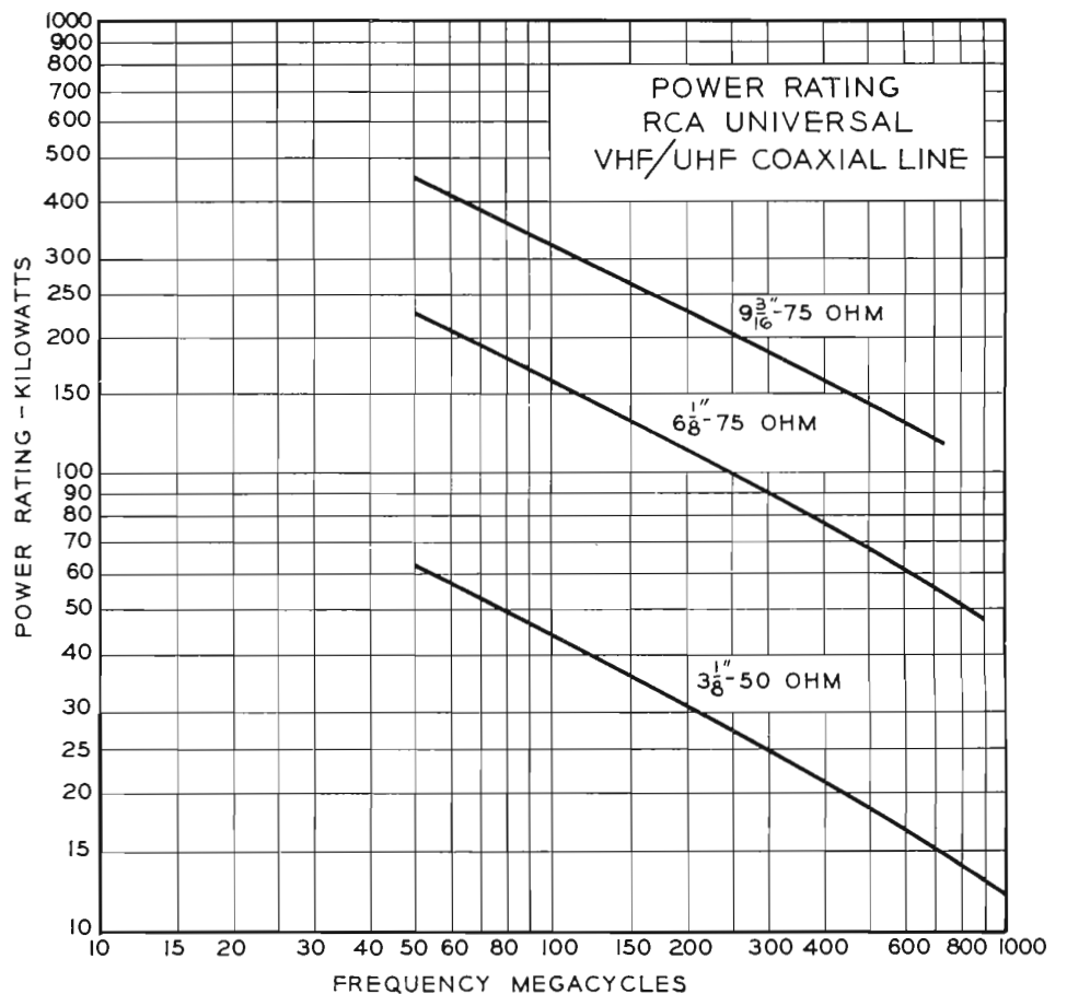
FIG. 6. The power ratings for universal transmission lines follow a descending curve as frequency is increased. The larger the size of the line the lower the attenuation per 100 feet.
