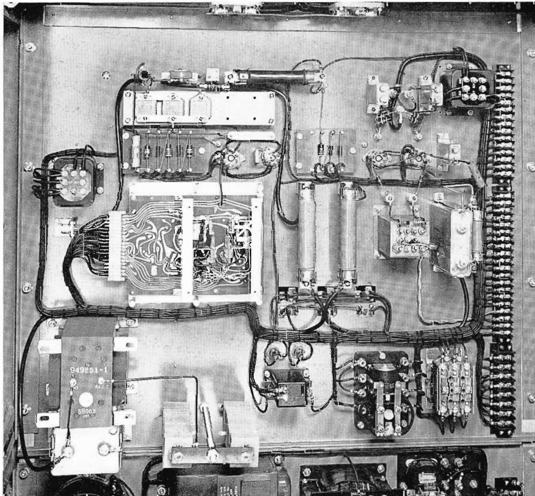
FIG. 8. The entire oscillator subassembly is shown from the rear. Vertical construction provides ease of maintenance. The oscillator chassis is easily removed with six thumbscrews. Note the convenient plug-in terminal strip on the oscillator chassis.
