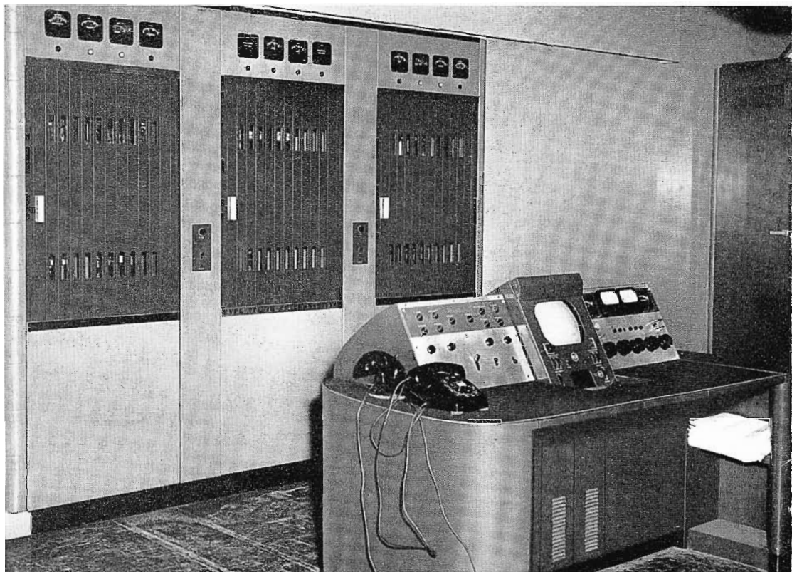
FIG. 7. Initial 1-kilowatt transmitter installation. A false wall provided room for expansion.
