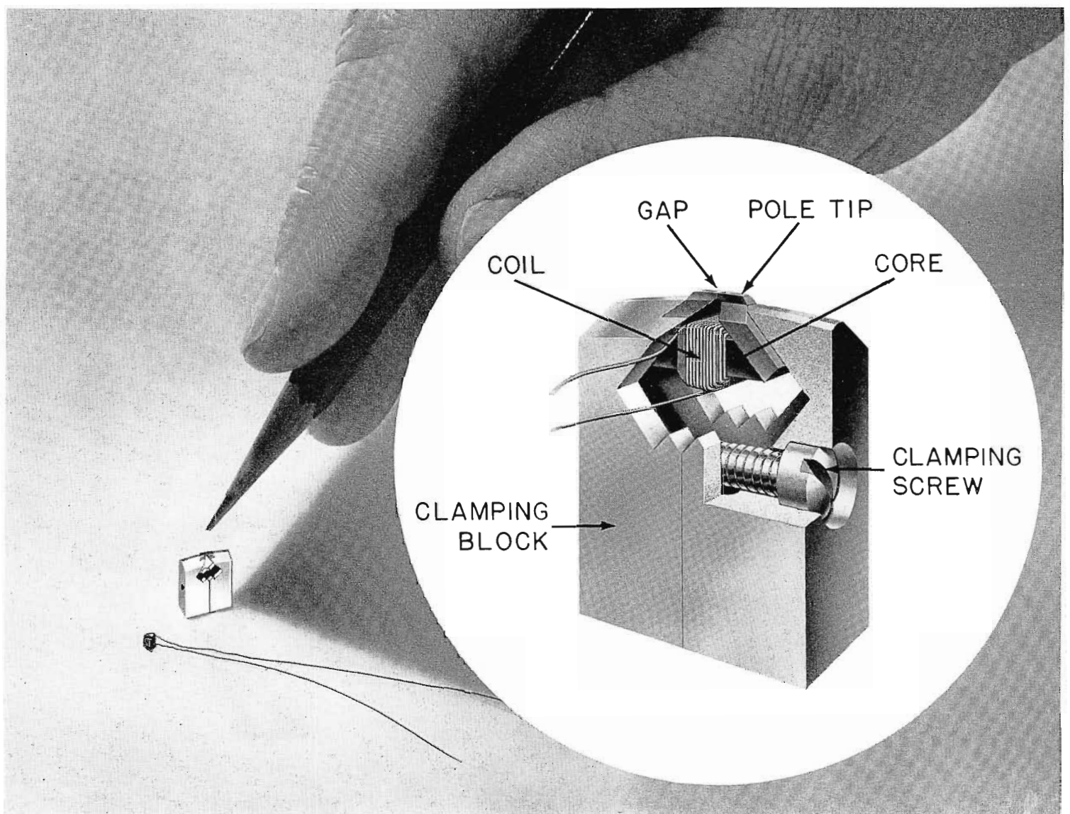
FIG. 5. Cutaway view showing details of a video recording head. Note size of head block, core and coil as compared with pencil.
