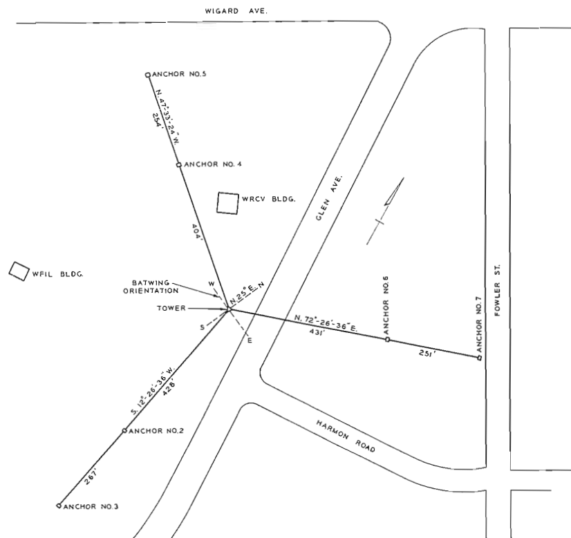
FIG. 7. Layout of WFIL and WRCV buildings with respect to the tower is shown.
