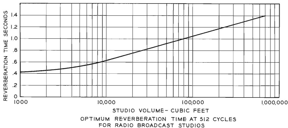
FIG. 5. This curve shows the variation in reverberation time as the size of the room increases with a 512-cycle reference signal.
