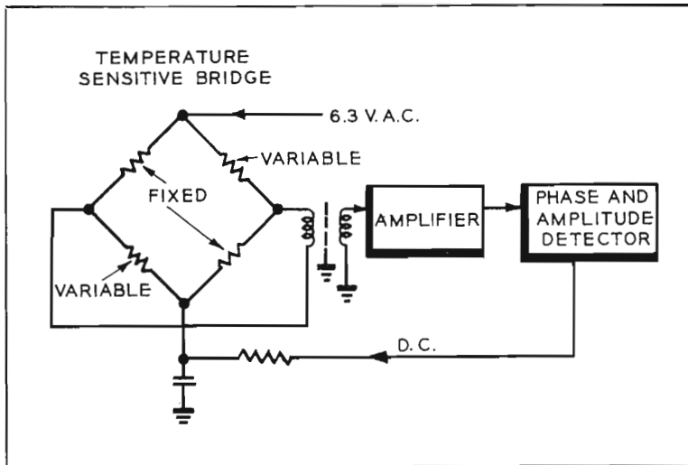
FIG. 5. Diagram of the oven-control circuit. Changes in ambient temperature unbalance the bridge and modify the power flow to keep the oven temperature constant.
