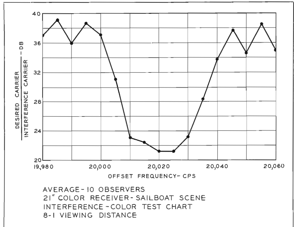
FIG. 3. Note the difference in db required to produce a tolerable picture with the carriers offset by 20 kc.
