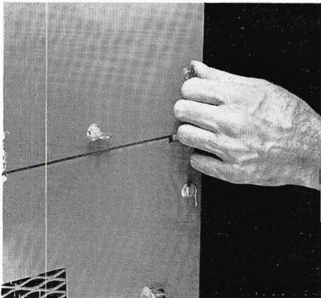
FIG. 3. The rear panels on the BTA-500R and 1R are easily removed with these thumbscrew fasteners to permit speedy access to all chassis.
