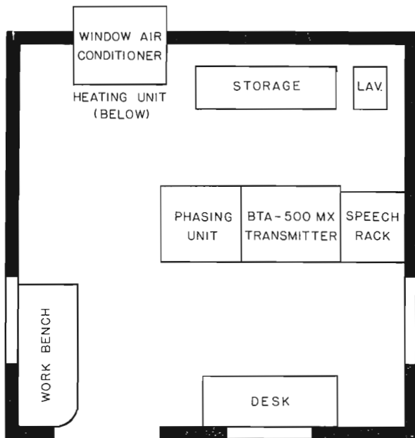
FIG. 14. Layout of KBKC transmitter building showing all facilities required for remote operation.
