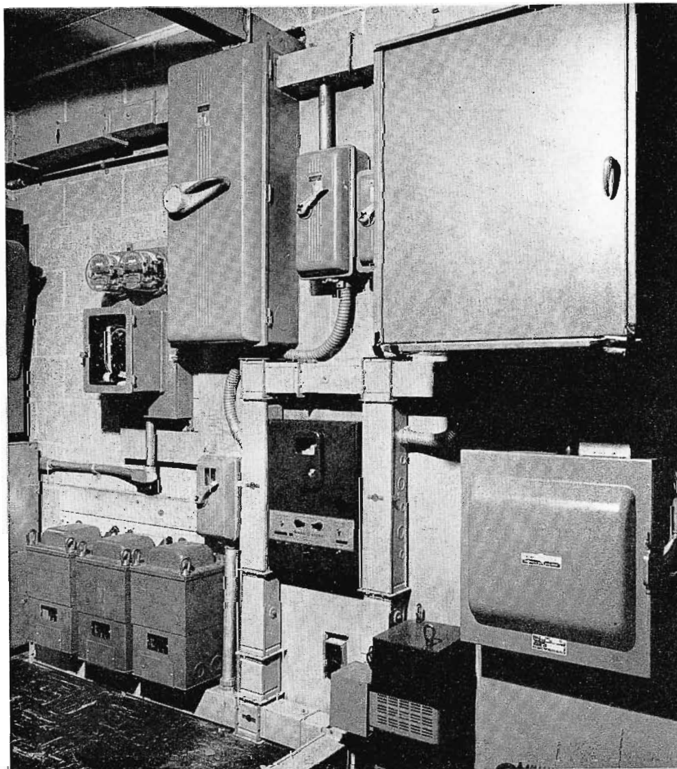
FIG. 4. Power equipment for operation of 25-kilowatt transmitter. Modifications called for changing primary service from 230 to 480 volts.
