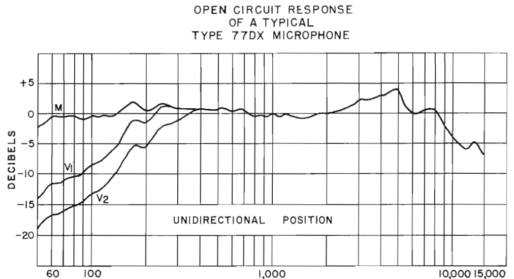
FIG. 7. This is the unidirectional response curve for the RCA Type 77-DX Microphone. A good microphone is necessary for combination control rooms.
