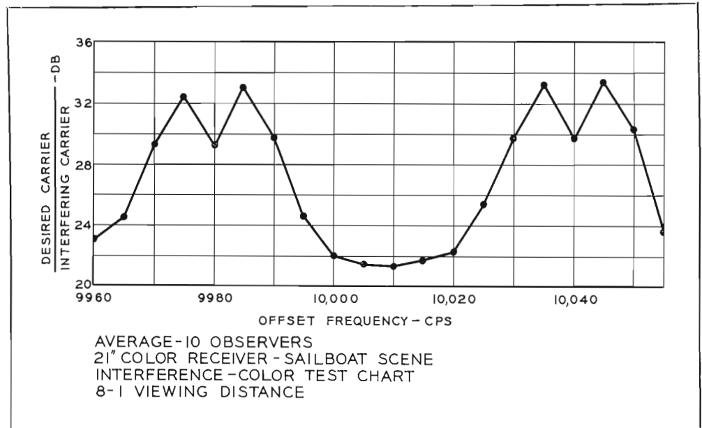
FIG. 2. The difference in db required to produce a tolerable picture with carriers offset by approximately 10 kc.
