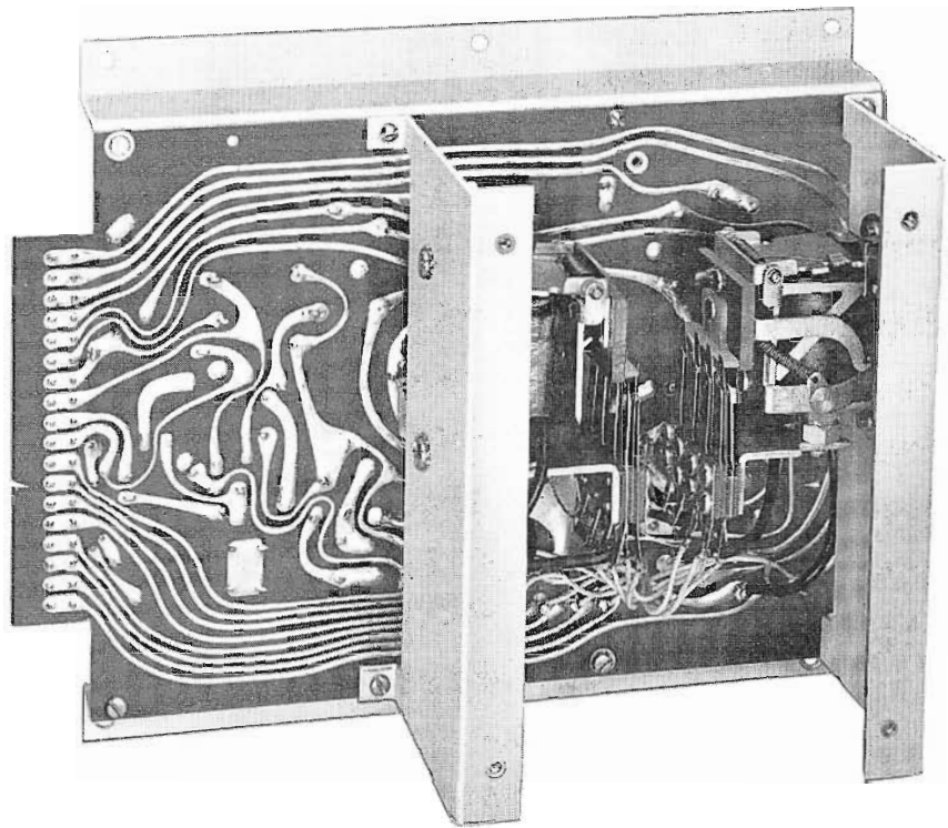
FIG. 7. The underside of the oscillator chassis is shown here. The relays are used to switch the crystals. Etched wiring simplifies servicing and also helps to improve oscillator stability.
