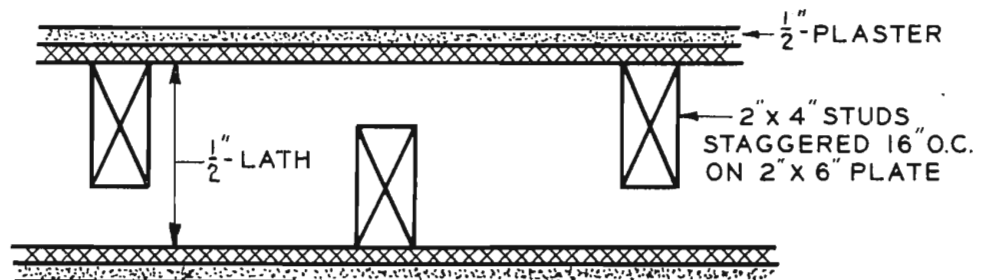
FIG. 1. This shows a cross section of a sound-insulating partition. Wooden walls should be constructed in this manner to reduce external noise.
