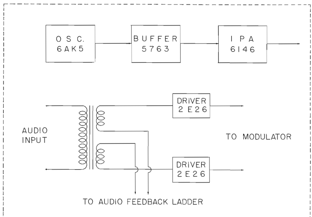
FIG. 6. The basic exciter subassembly is shown in this block diagram. Only three RF tubes are used, and the modulator input uses two tubes.
