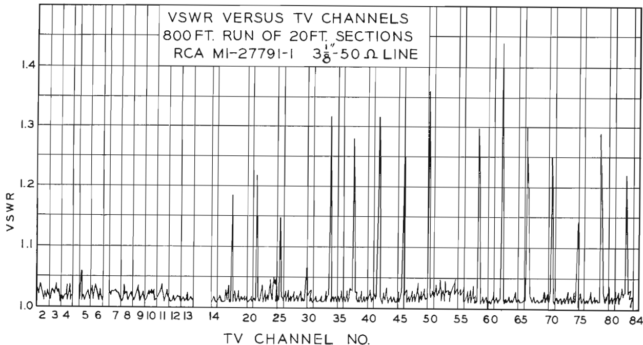
FIG. 7. The VSWR peaks on long runs of line at frequencies where 20-foot sections are an integral of half a wavelength. Spikes can be avoided by using 19½-foot sections.
