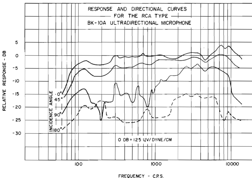
FIG. 3. The frequency response curves for the BK-10A are shown for various incidence angles of sound pickup.
