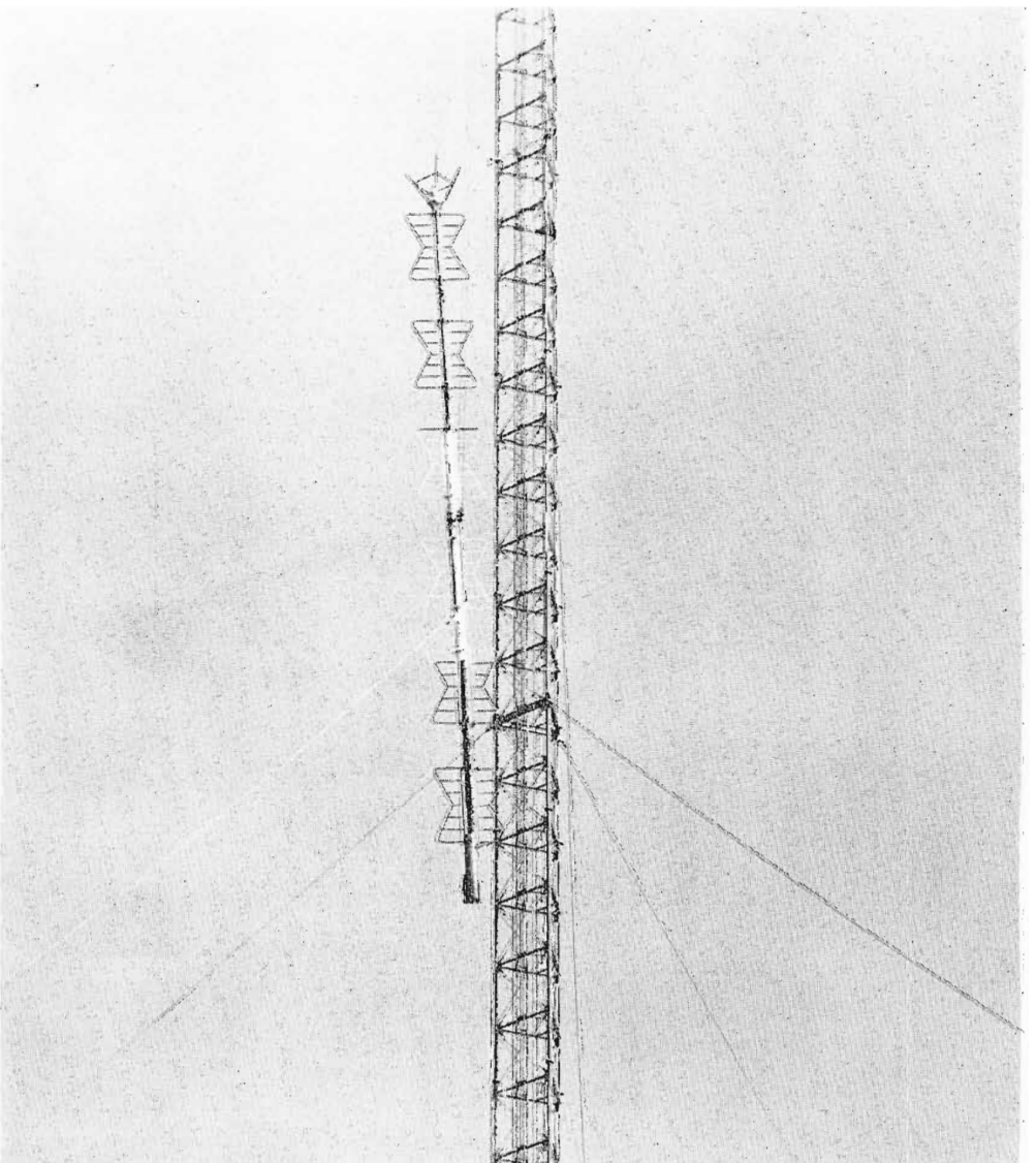
FIG. 3. The WFIL-TV Type TF-6BM Superturnstile Antenna being raised to top of tower. Note the 1000-watt beacon on top of the antenna structure.
