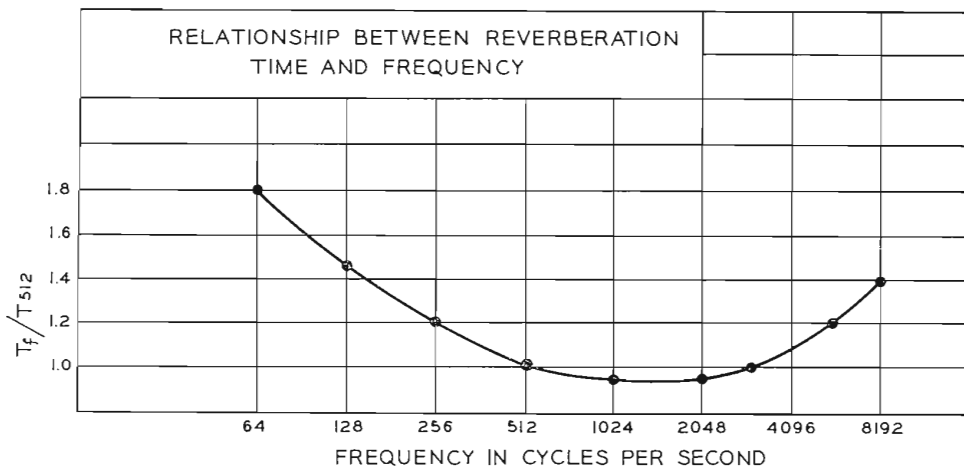
FIG. 4. These Morris-Nixon curves show the relationship between the reverberation time and the frequency. Reverberation time should remain fairly constant between 100 and 5000 cycles.
