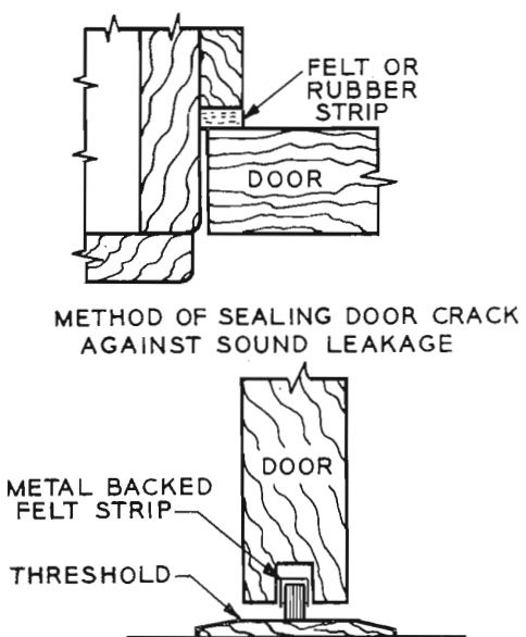
FIG. 2. Here are the normal methods for sealing the control-room door. The door itself should be of the heavy type to improve isolation of the control room.
