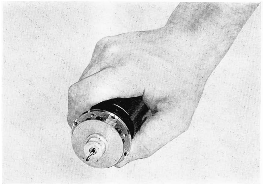
FIG. 4. Close-up of the video head wheel. Four video recording heads are located 90 degrees apart around the head wheel.
