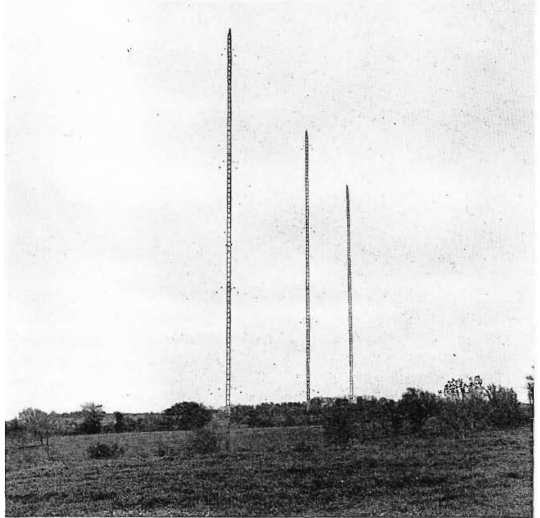
FIG. 15. Three-tower directional antenna system designed to cover Kansas City area. Towers are 185-ft. high, insulated guyed affairs.
