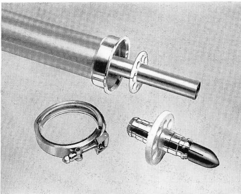
FIG. 1. A view of the 3\frac{1}{8} -inch Universal Transmission Line showing inner conductor, support insulator, Marman clamp, and the inner conductor anchor insulator.
