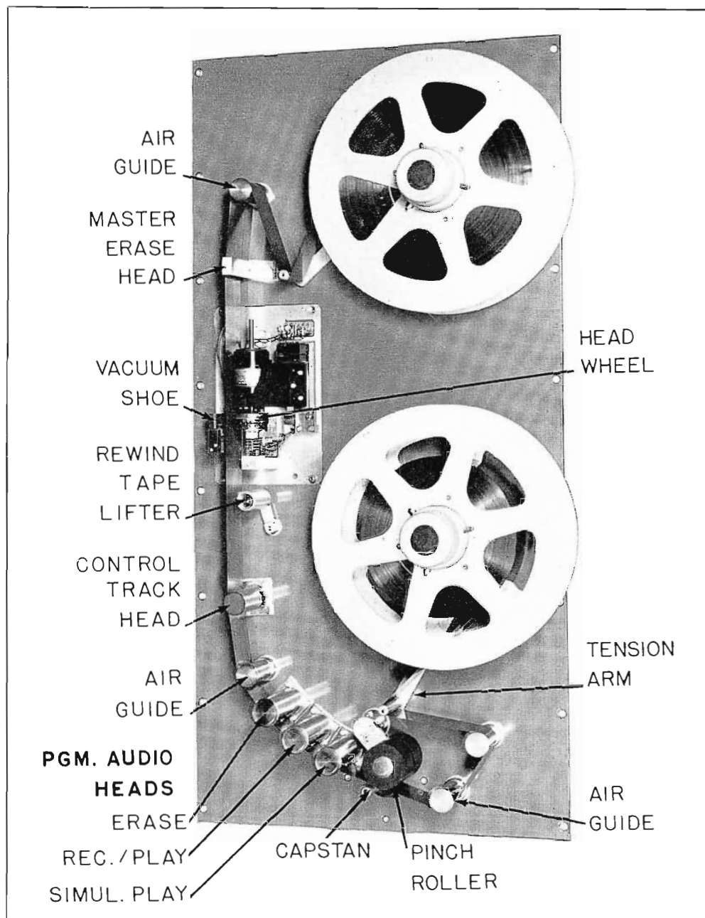
FIG. 7. Close-up of the tape transport mechanism. Call-offs identify key components for record and playback functions.
