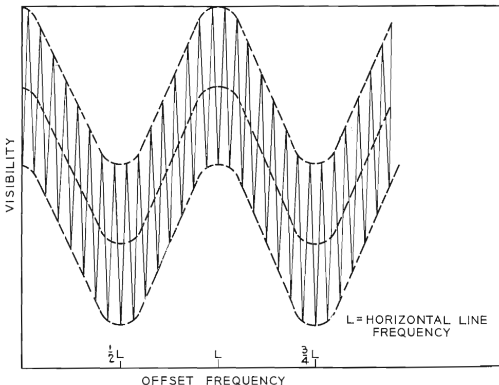
FIG. 1. The offset of cochannel visual carriers is shown; note the fine structure that is superimposed. The maxima and minima points occur at multiples of one-half the line frequency.
