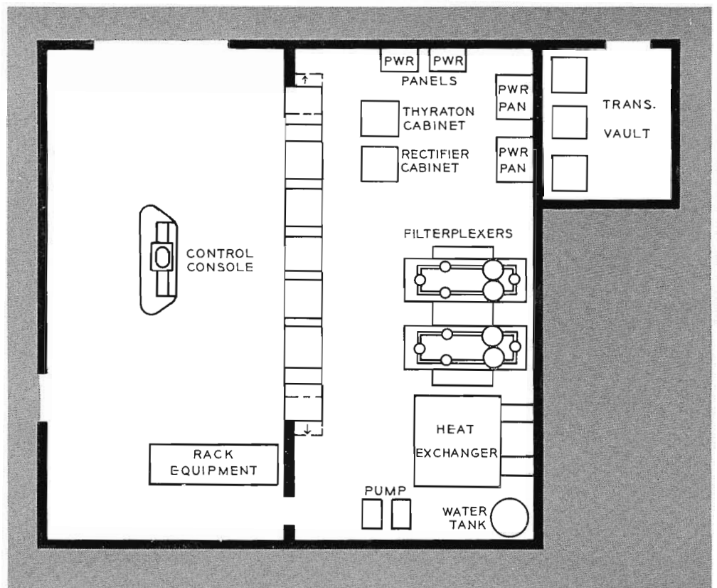
FIG. 6. Block diagram showing how modifications from 1 to 12 to 25 kilowatt transmitter were accomplished without additions to the building.
