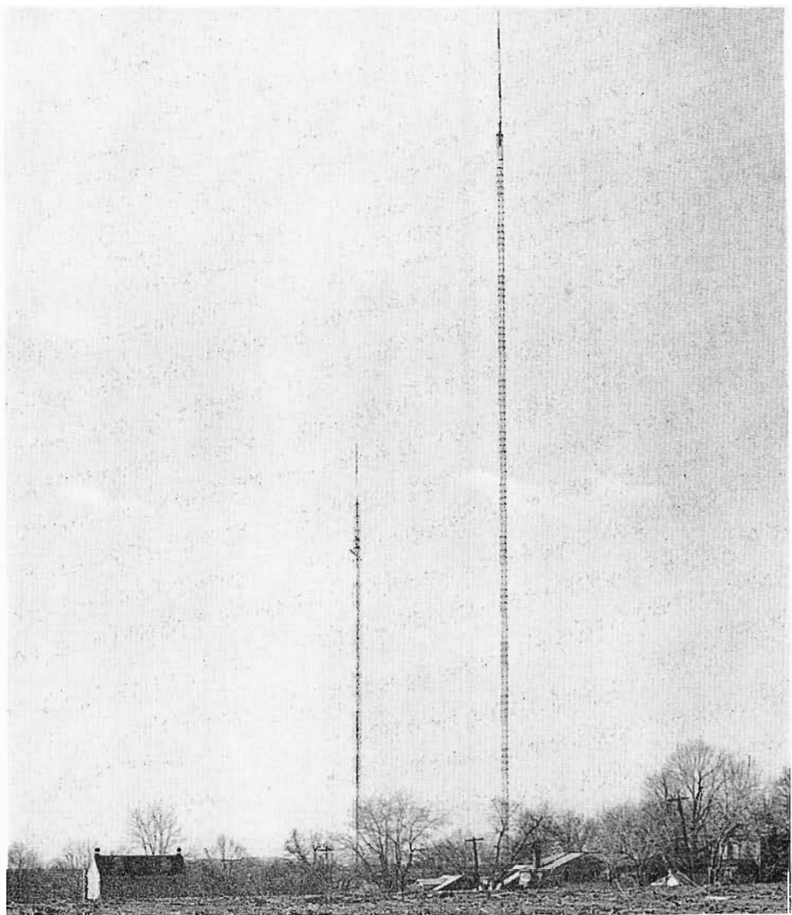
FIG. 2. The new 1109-foot tower is shown in comparison to WFIL's former tower structure.
