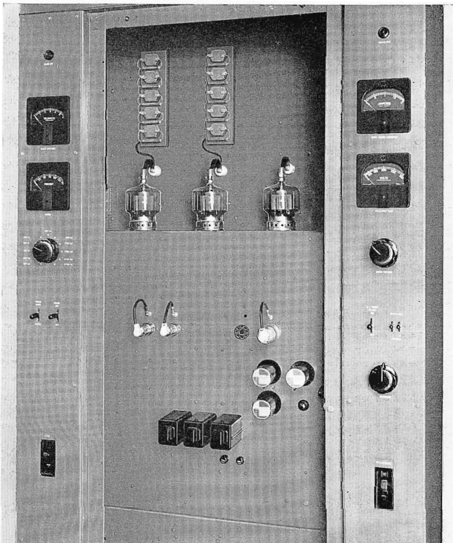
FIG. 11. Front of BTA-500 new transmitter permits easy tube change. Power amplifier and modulator tubes are located on the top chassis, and just below this is the exciter chassis. All normal operating controls are shown on the two side panels.
