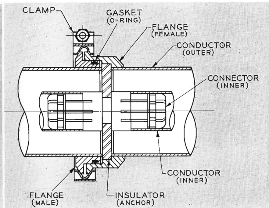
FIG. 2. This is a cutaway drawing showing the flanged connector assembly of the Universal Transmission Line.
