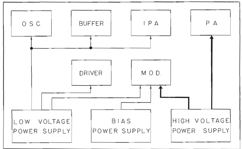
FIG. 10. This block diagram shows the power supplies. The low voltage and bias power supplies use selenium dry-disc rectifiers, while the high voltage supply uses two.
