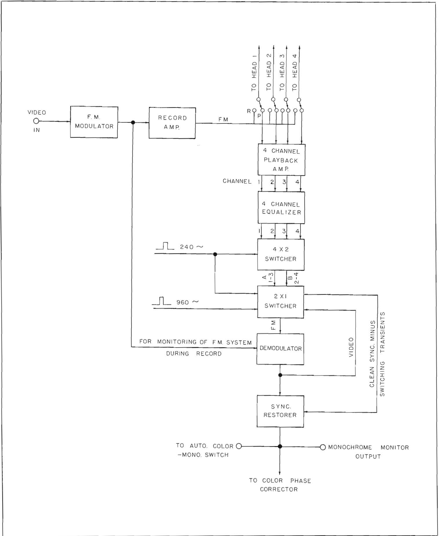
FIG. 9. Functional diagram showing the details of the video system block of Fig. 8.
