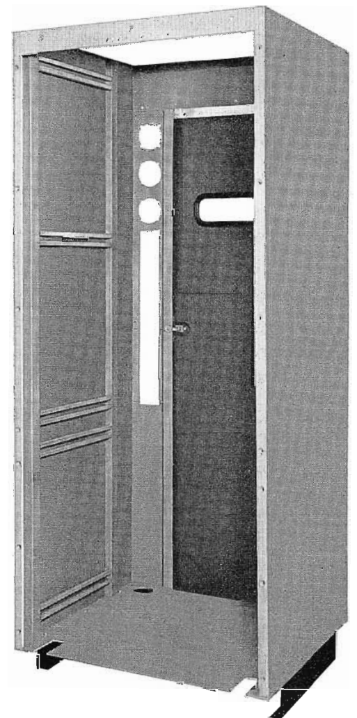
FIG. 12. The transmitter cabinet is made of aluminized-steel for better shielding and strength. The rigid construction is shown here; note the additional supports across the side of the cabinet.
