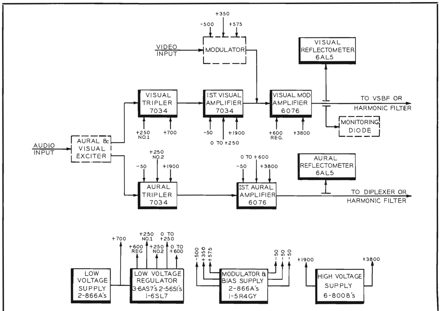
FIG. 5. A block diagram of the TT-2BH 2-KW TV Transmitter.
