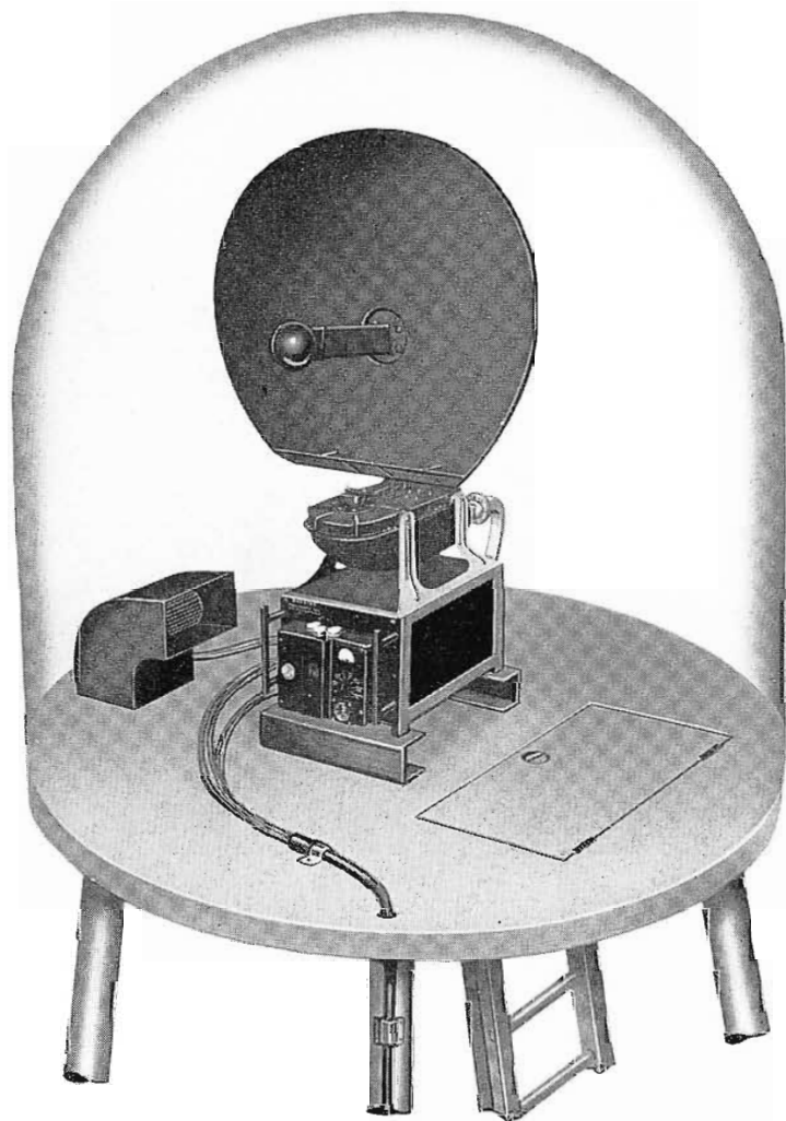
FIG. 1. The radome is about five feet in diameter and six feet in height and may be mounted on a building or tower. Here is located antenna and receiver-transmitter. Radome also contains provisions for a blower-heater unit to prevent moisture condensation and facilitate cooling.
