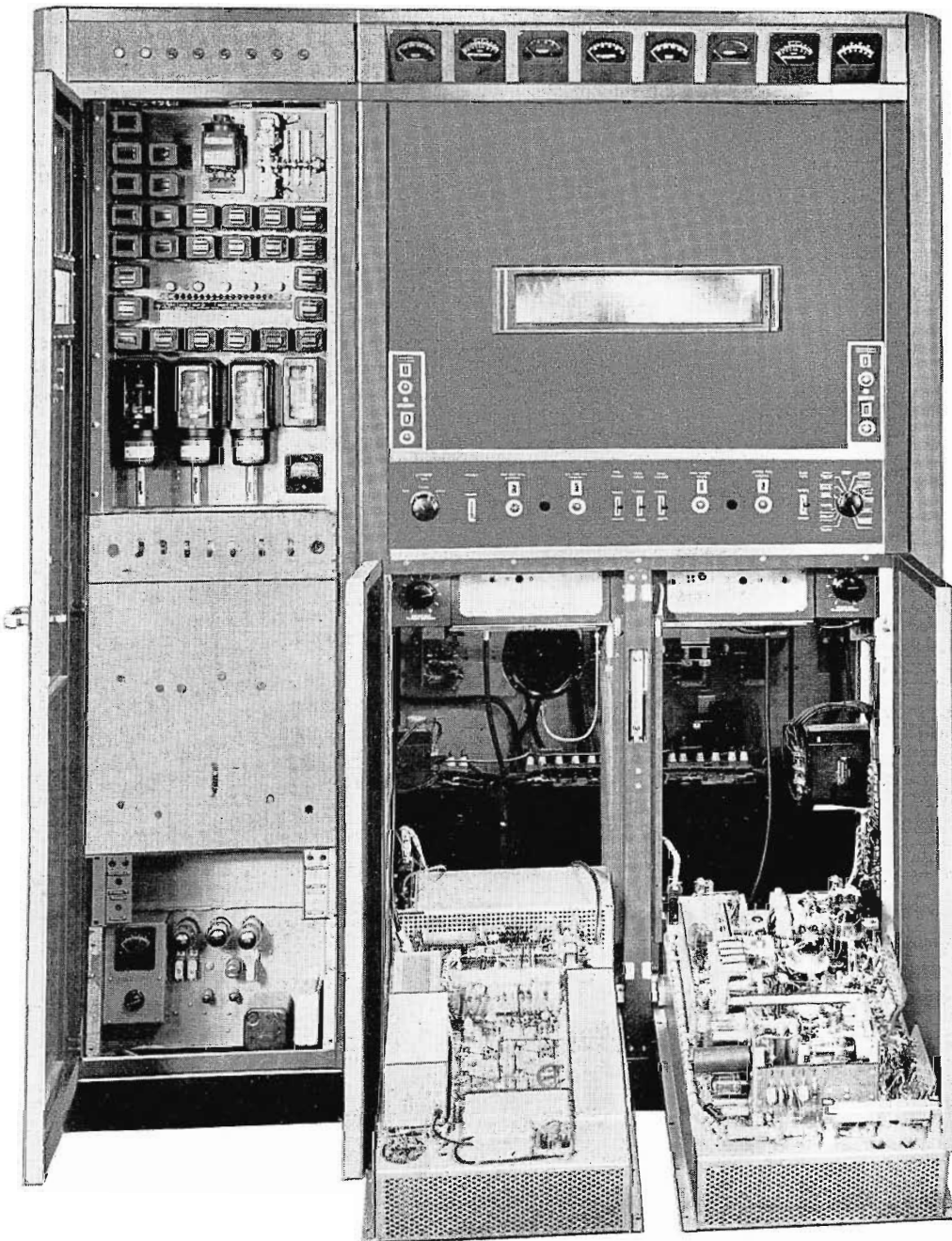
FIG. 6. Note "Dutch door" design of TT-2BH transmitter. The modulator and exciter tilt out for ease of servicing.
