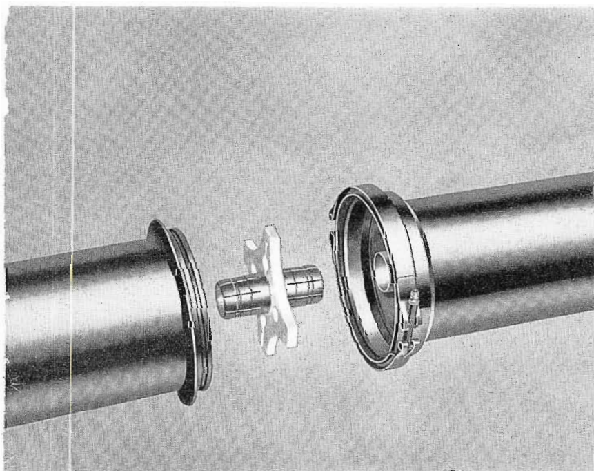
FIG. 3. An exploded view of the flange connector on a section of \frac{9}{16} -inch Universal Transmission Line.
