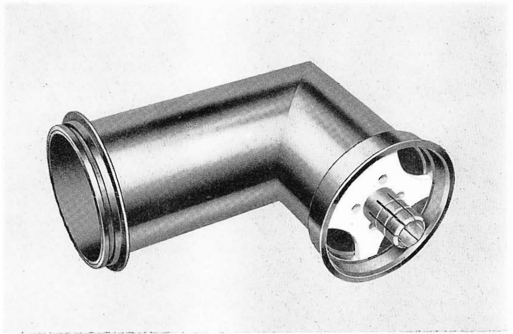
FIG. 9. A 90-degree miter elbow for 6 1/8-inch Universal Transmission Line is shown with its inner conductor and Teflon insulator.
