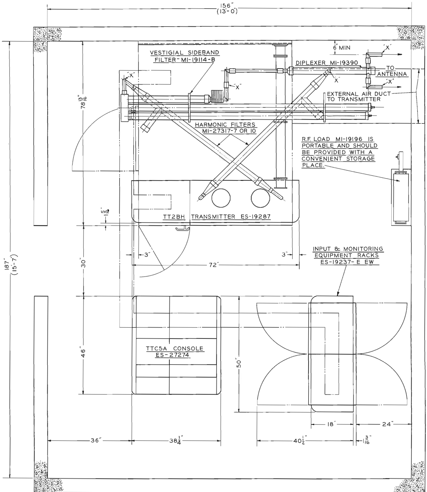
FIG. 2. Typical floor plan arrangement for the TT-2BH. The entire transmitter is only 72 inches wide and can be located in a small floor area. At points marked by "X," provisions should be made for connection of a dummy load for testing and tuning the TT-2BH.
