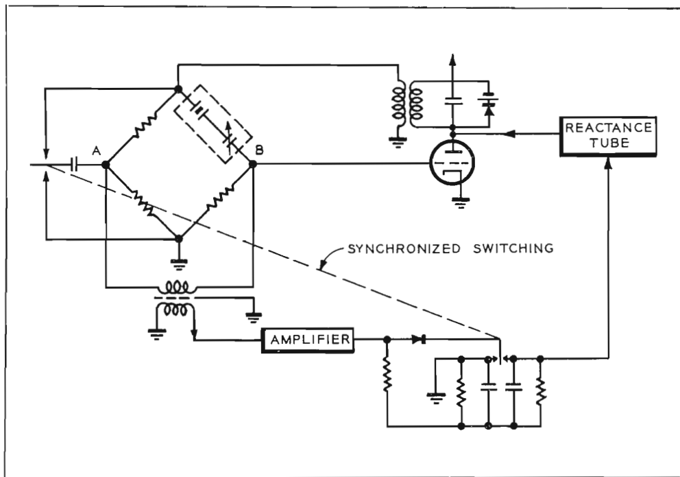
FIG. 4. Here is an oscillator circuit that is stable enough to produce the required frequency control tolerances.
