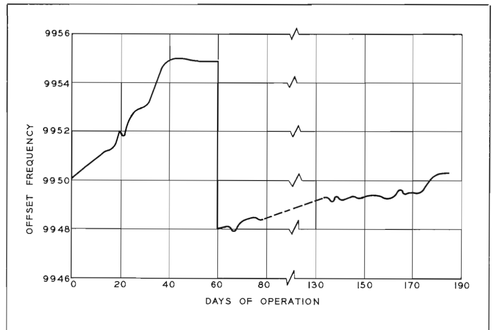
FIG. 6. Actual field tests were made with this system, and this graph indicates the relative stability obtained.
