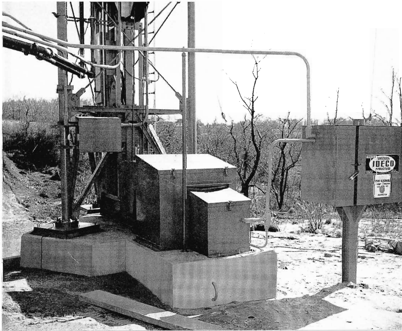
FIG. 5. Another view of the foundation showing the transmission line feed from WRCV. Cabinet at right contains the tower-lighting control and the radio-control unit for the two-man elevator.
