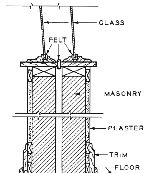
FIG. 3. Sound-insulating window construction showing structural separation of double wall. Glass windows in studios and control rooms should be offset about 10 degrees, and they should be mounted as shown on a double wall.
