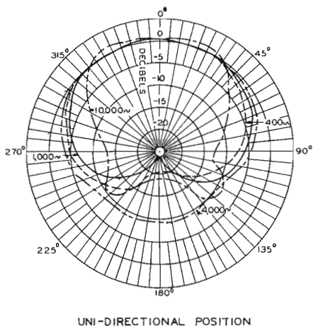
FIG. 7. This is the unidirectional response curve for the RCA Type 77-DX Microphone. A good microphone is necessary for combination control rooms.
