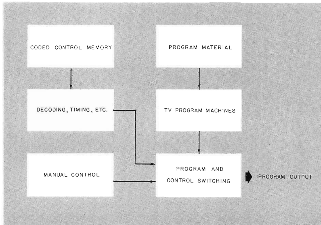
FIG. 5. Functional diagram of automatic control system showing relationship of memory and timing devices to basic program equipment.
